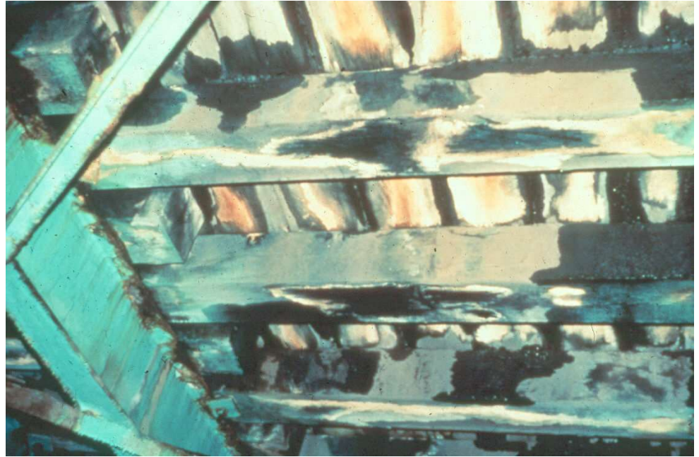
Figure 6.1.9 Mold and Stain on Underside of Timber Bridge
