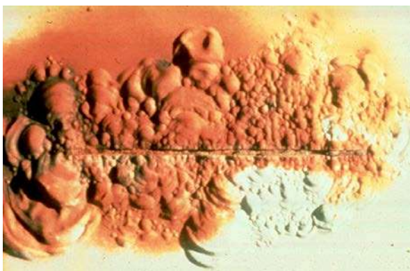
Figure 6.3.16 Rust Undercutting at Scratched Area
