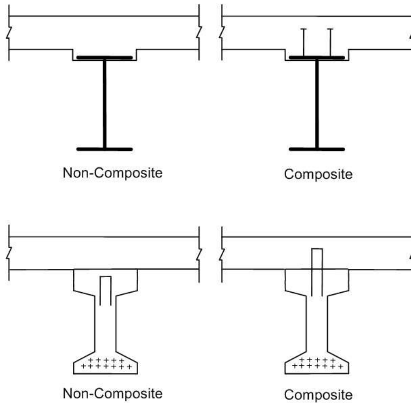
Figure 5.1.25 Non-Composite or Composite Concrete Deck on Steel Beams and Prestressed Concrete Beams
