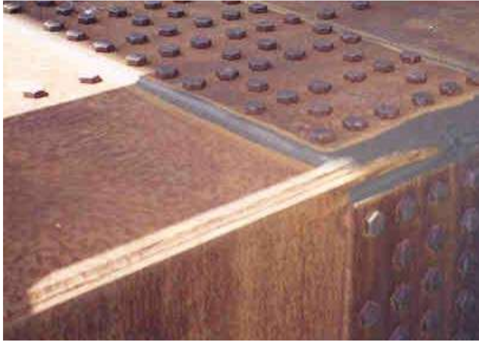
Figure 6.3.28 Light Brown – Early Development of the Oxide Film (Patina)
