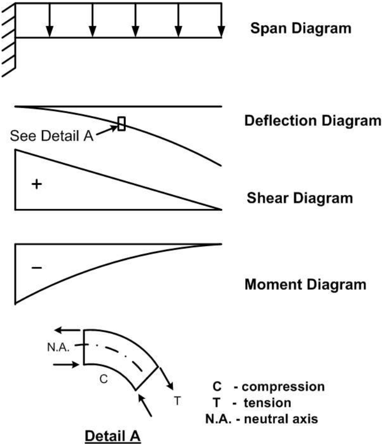
Figure 5.1.23 Cantilever Span
