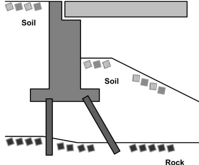
Figure 5.1.30 Deep Foundation
