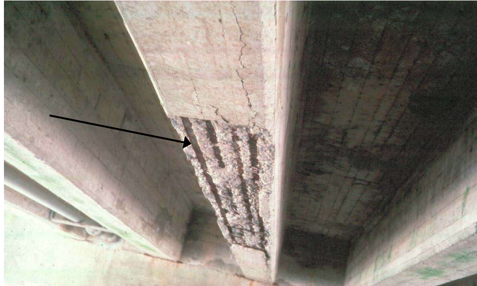
Figure 6.2.5 Concrete Member with Tensile Steel Reinforcement Showing
