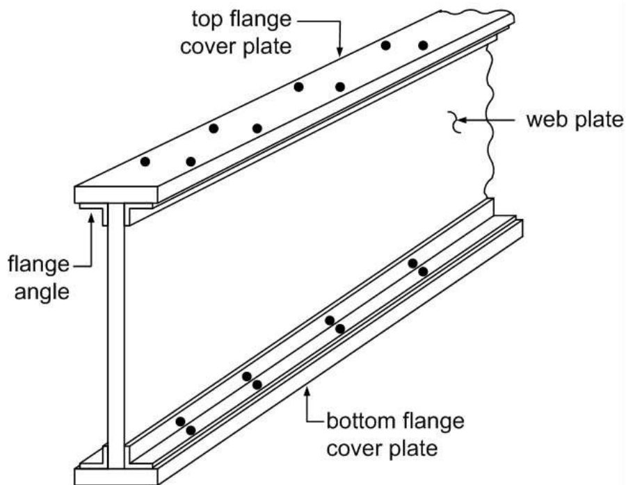
Figure 6.4.6 Internally Redundant Riveted I-Beam
