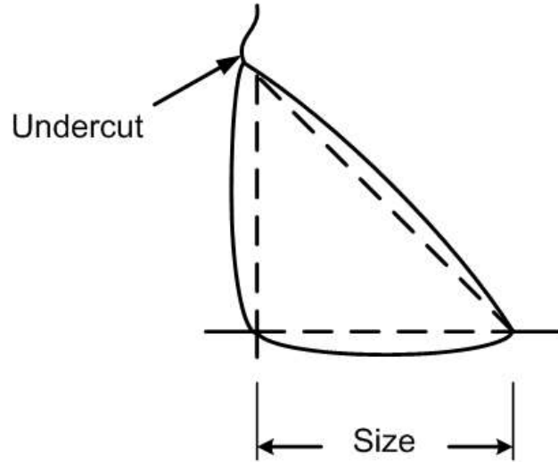
Figure 6.4.25 Undercut of a Fillet Weld
