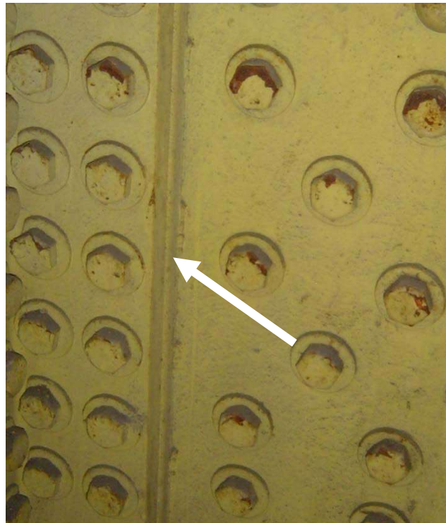
Figure 6.4.16 Tack Weld
